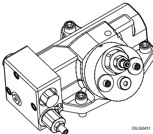
Figure 1. Typical Oilgear Type “P-1NN/H” Single Pressure Compensator Control w/Horsepower Limiter, F1U Series Control for “PVG” -048/-065/-075 B-Frame Pumps
