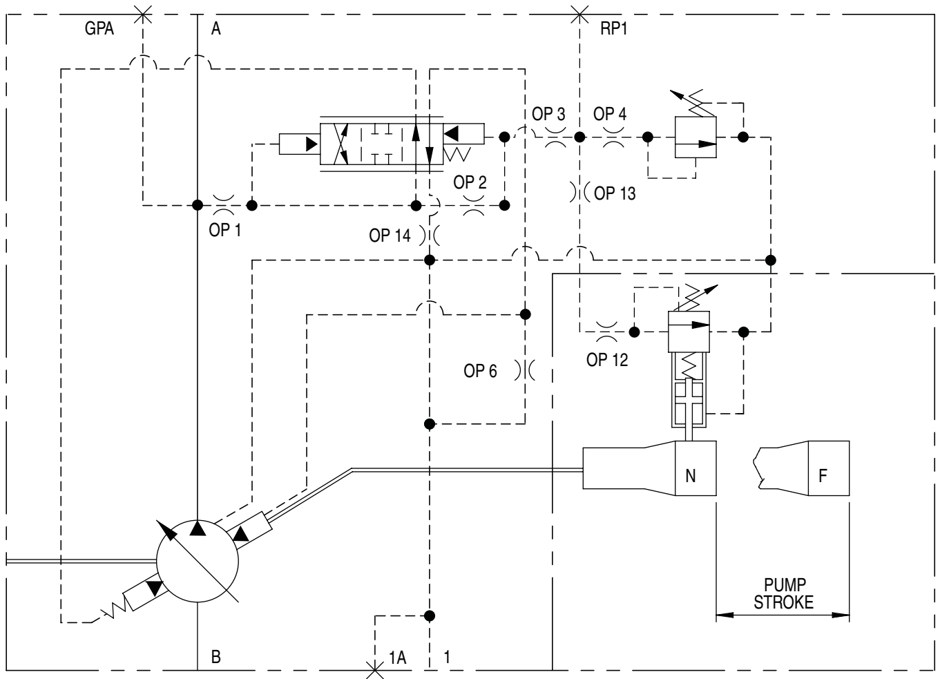
Figure 2. ASA Diagram for “P-1NN/H” Control Shown with Typical Pump
