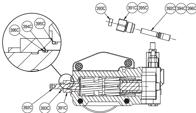
Figure 8. Exploded Parts Drawing for "P-CNN/H" Maximum Volume Stop, Series F1U Control
