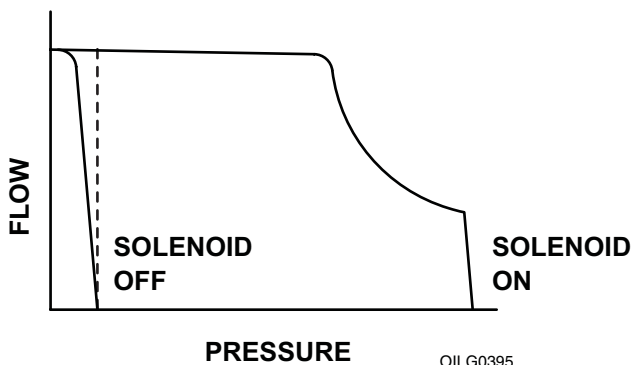
Figure 3. Curve Indicating Flow Versus Pressure for "P-CNN/H" Type Control
