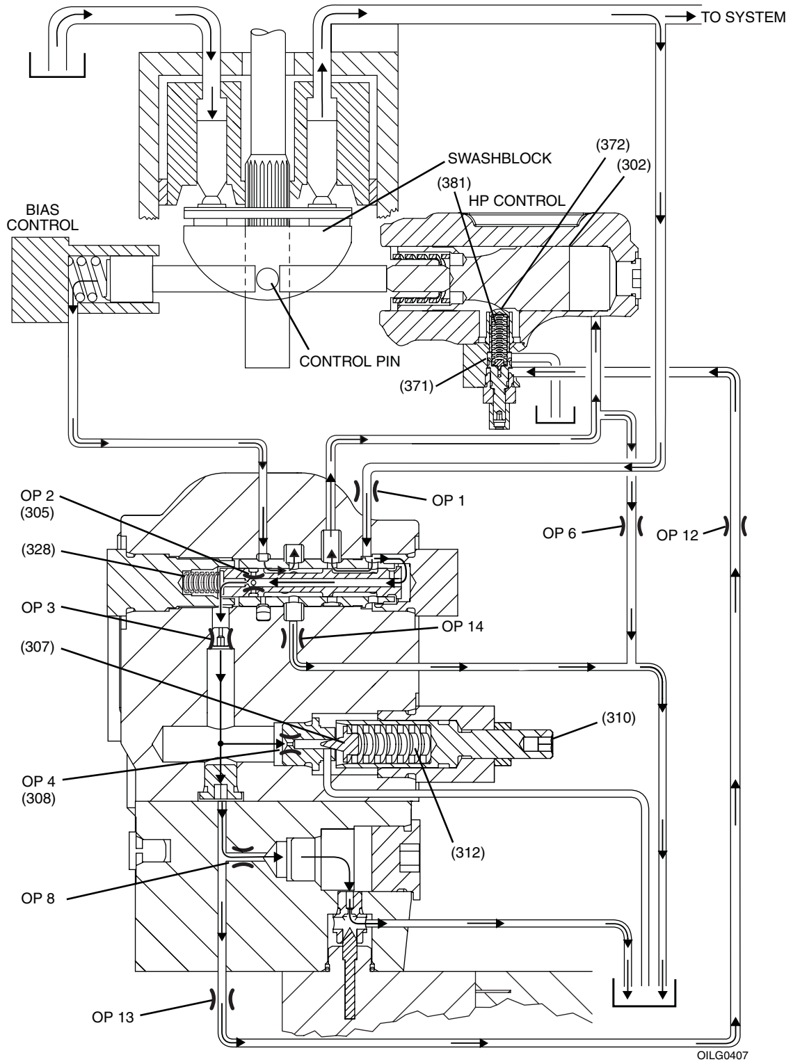
Figure 5. Compensating Pressure (Unloading) at Minimum Pressure with Pilot Vent Valve Deenergized to Pass Flow
