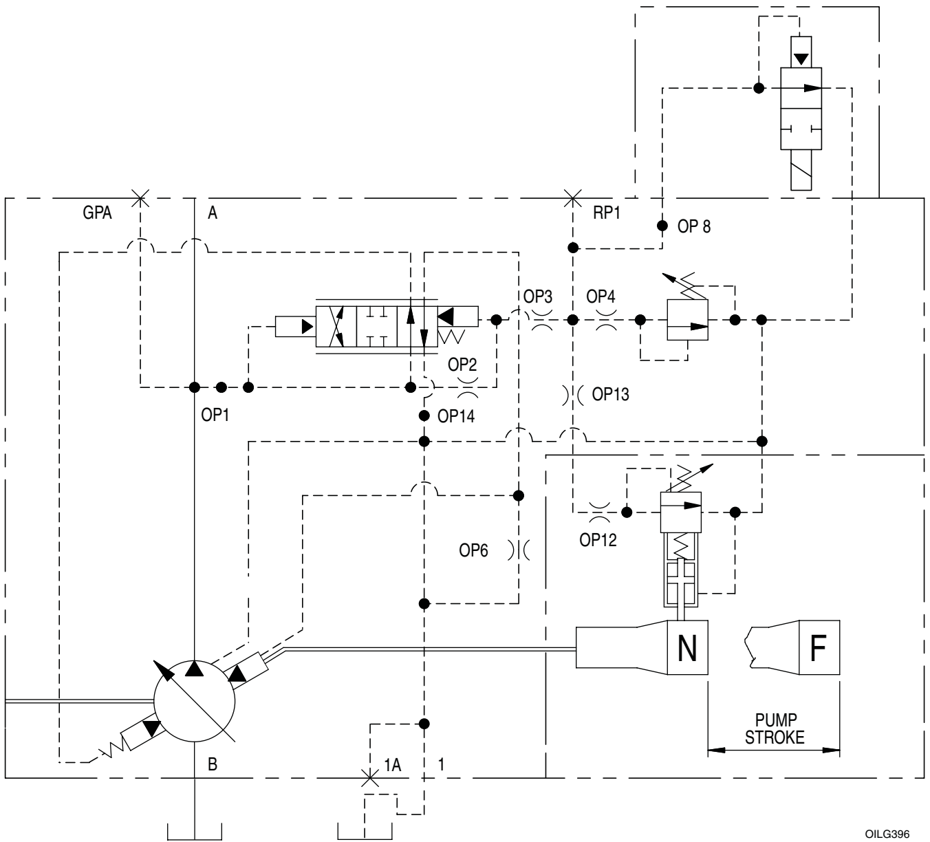
Figure 2. ASA Diagram for "P-CNN/H" Control Shown with Typical Pump
