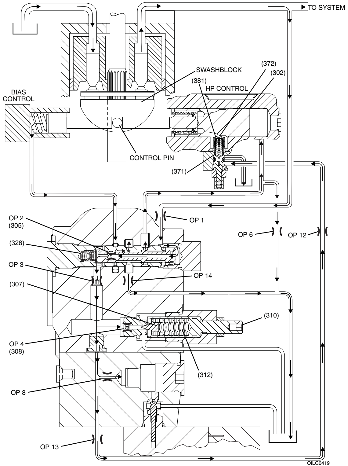
Figure 7. Compensating Pressure (Unloading) - Horsepower Limiter Active
