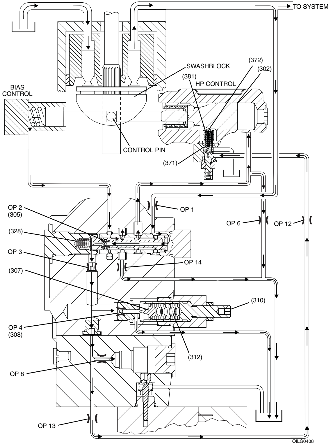
Figure 6. Compensating Pressure (Unloading) at Higher Pressure with Pilot Vent Valve Energized to Block Flow
