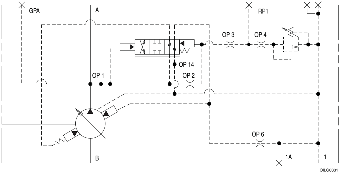
Figure 2. ASA Diagram for "P-1NN" Control Shown with Typical Pump
