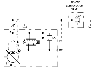
PUMP WITH REMOTE PRESSURE CONTROL
